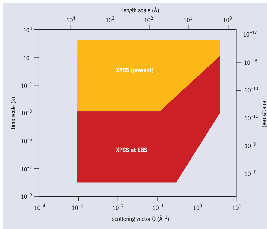
In XPCS, coherent light scattering from a sample forms a speckle pattern that reveals information about the intrinsic dynamics. Above: The dynamical range of XPCS before and after the EBS upgrade. Below: With the new EBSL1 beamline, the acquisition time ( \tau ) between speckle patterns will be 10,000 times faster, allowing the observation of much more rapid dynamical processes.
